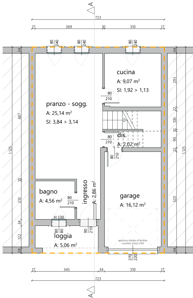
SdF piano terra 1:100
